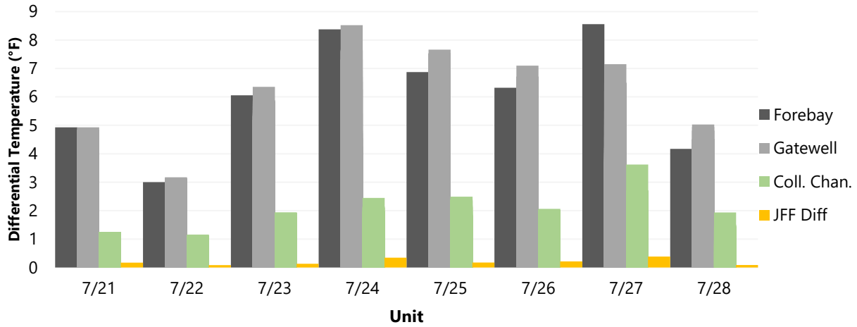
Figure 3 Average Weekly Water Temperatures by Position for Five Dam Locations from July 22 to July 28
